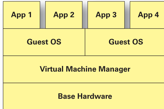
Figure 2 - Server Virtualization
